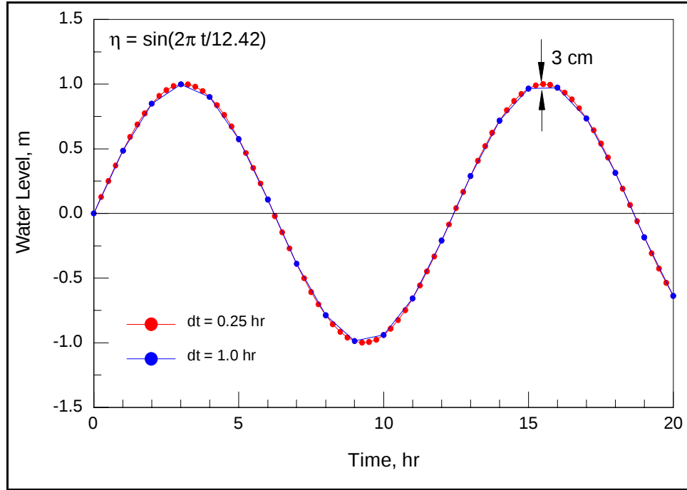
Figure 13. Time discretization of a sinusoidal water-level curve
